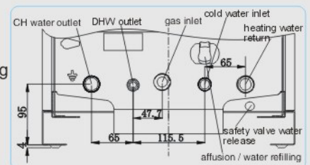
connector drawing (unit: mm)
